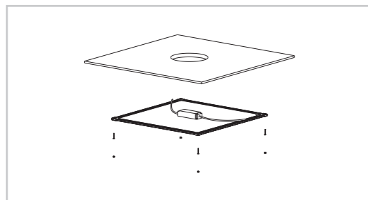
Hole Mounted
