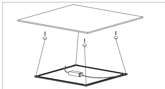
Suspended
