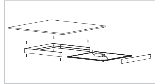
Surface Mounted with Bracket
