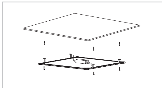
Surface Mounted with L-Shape Hinges
